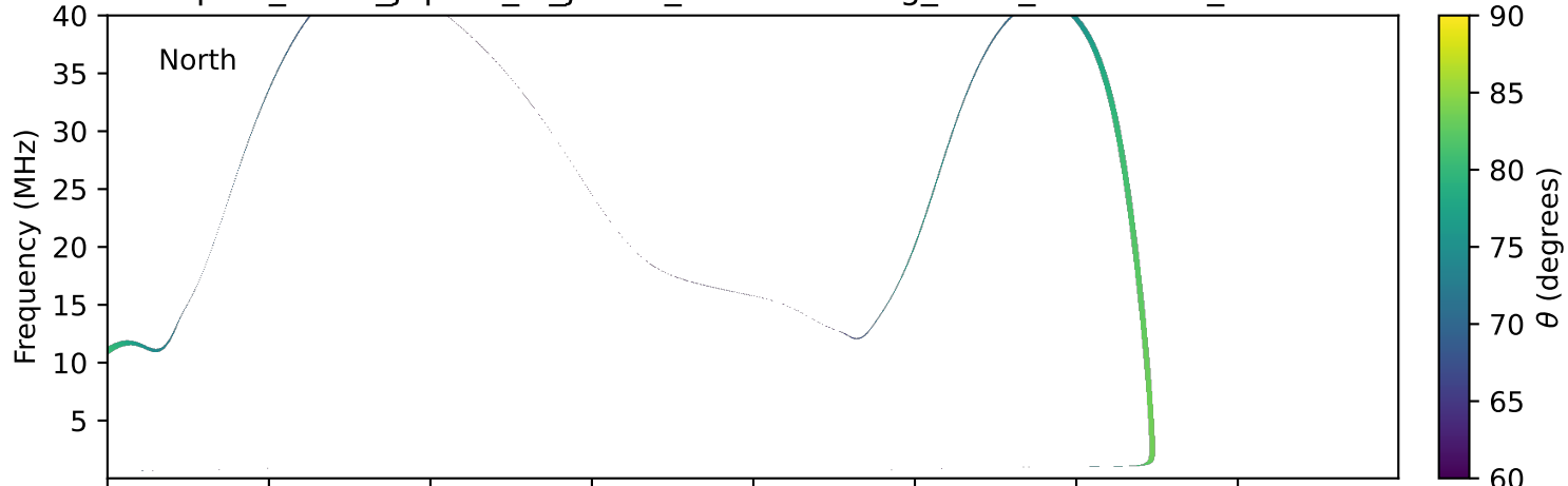
expres_earth_jupiter_io_jrm09_lossc-wid1deg_3kev_19990602_v11.cdf
