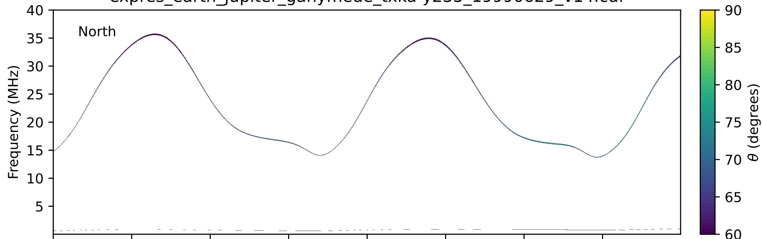
expres_earth_jupiter_ganymede_txka-y235_19990629_v14.cdf
