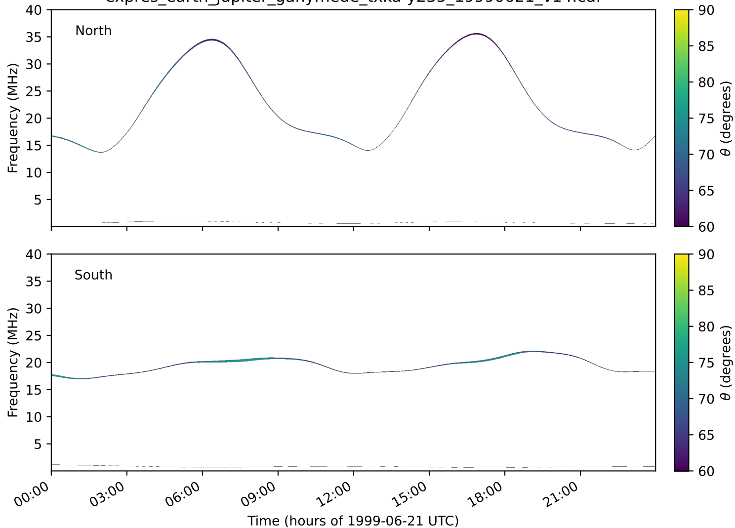
expres_earth_jupiter_ganymede_txka-y235_19990621_v14.cdf
