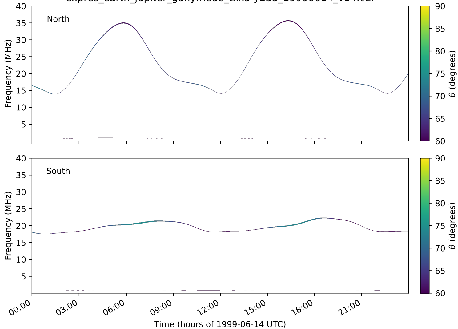
expres_earth_jupiter_ganymede_txka-y235_19990614_v14.cdf
