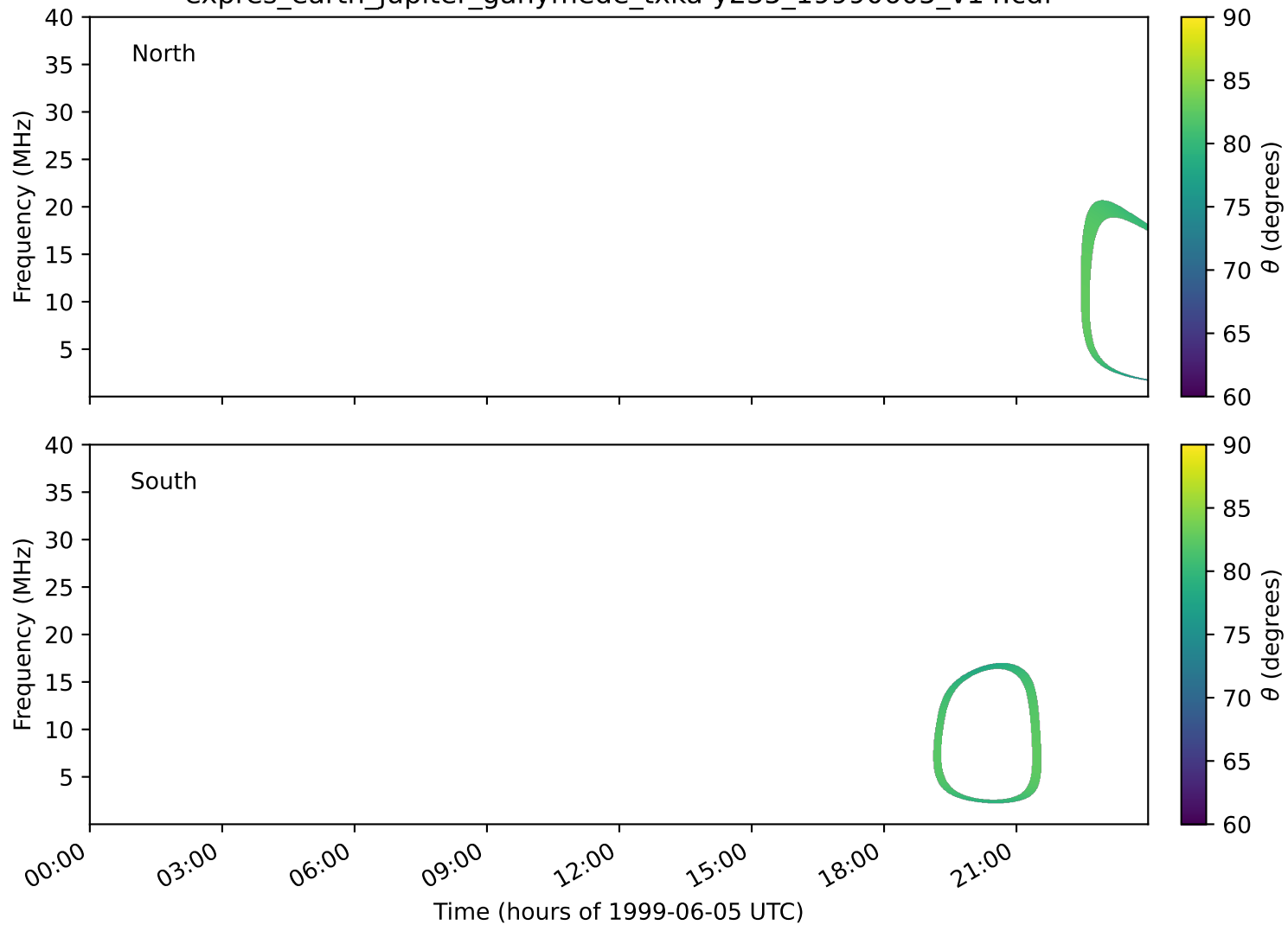
expres_earth_jupiter_ganymede_txka-y235_19990605_v14.cdf
