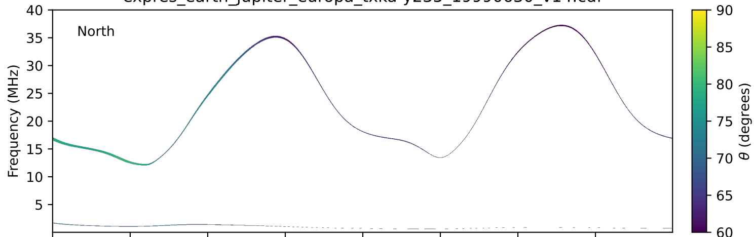
expres_earth_jupiter_europa_txka-y235_19990630_v14.cdf
