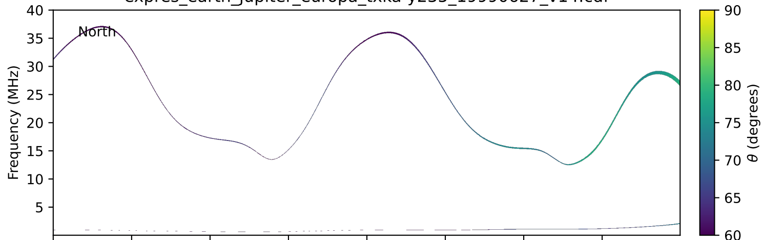
expres_earth_jupiter_europa_txka-y235_19990627_v14.cdf
