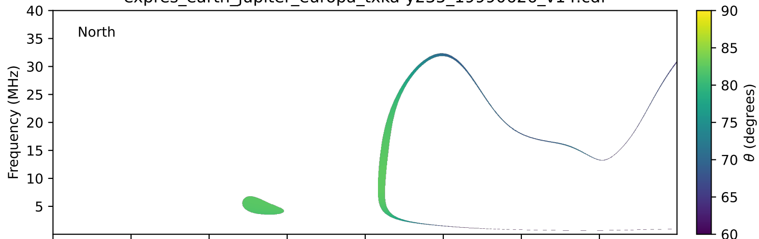
expres_earth_jupiter_europa_txka-y235_19990626_v14.cdf
