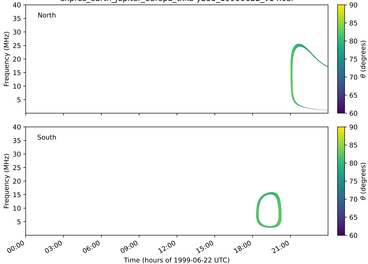
expres_earth_jupiter_europa_txka-y235_19990622_v14.cdf
