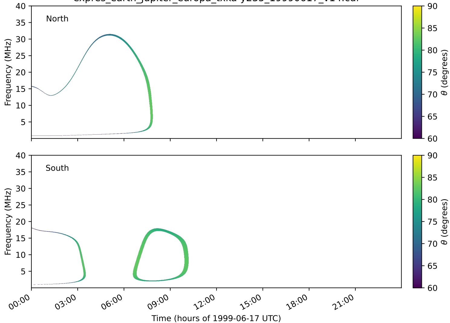
expres_earth_jupiter_europa_txka-y235_19990617_v14.cdf
