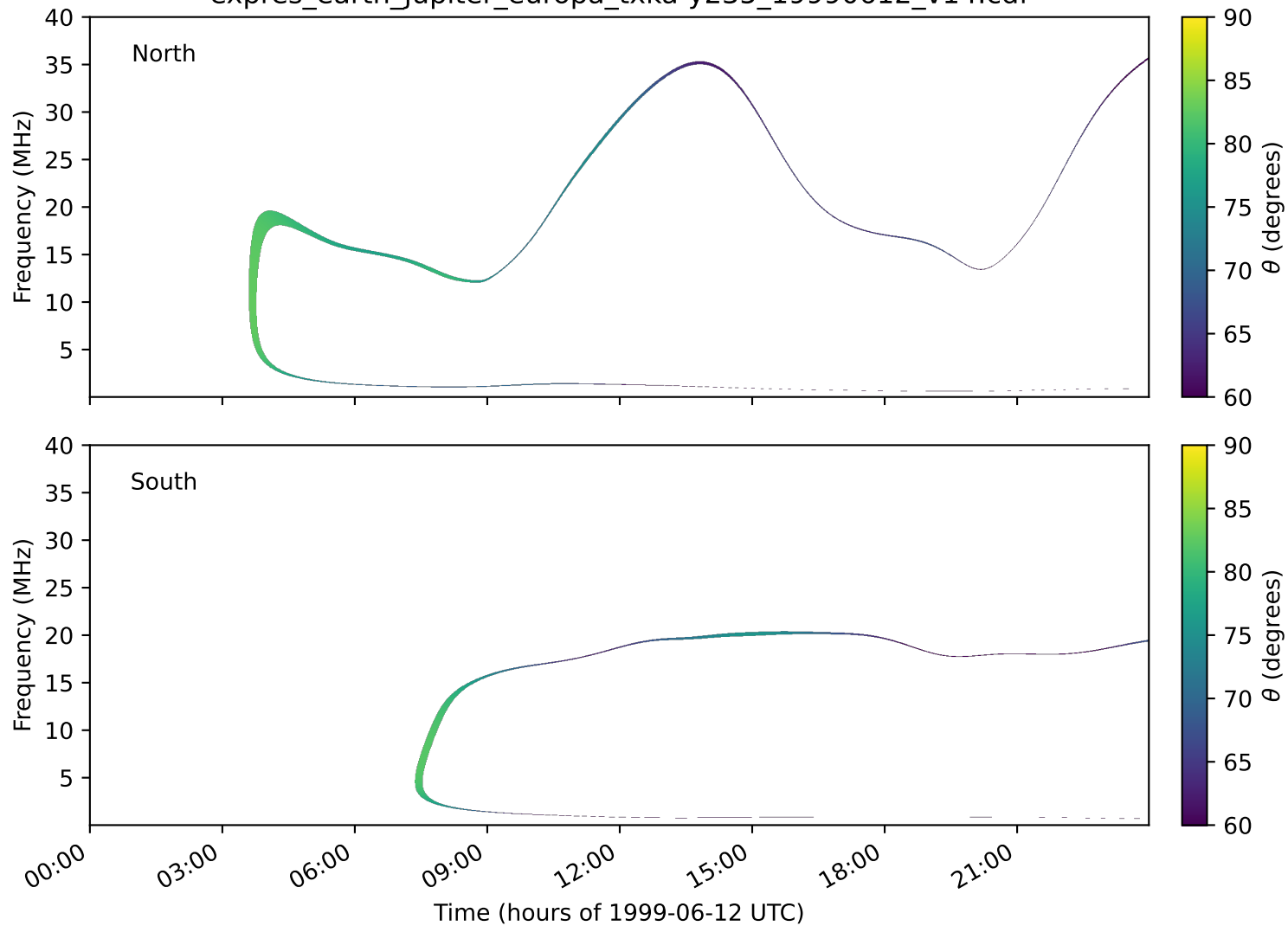
expres_earth_jupiter_europa_txka-y235_19990612_v14.cdf
