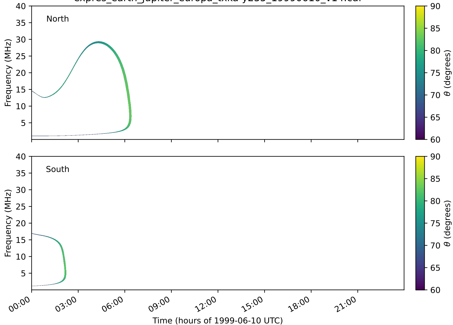
expres_earth_jupiter_europa_txka-y235_19990610_v14.cdf
