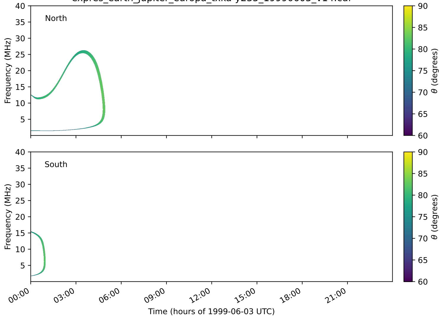
expres_earth_jupiter_europa_txka-y235_19990603_v14.cdf
