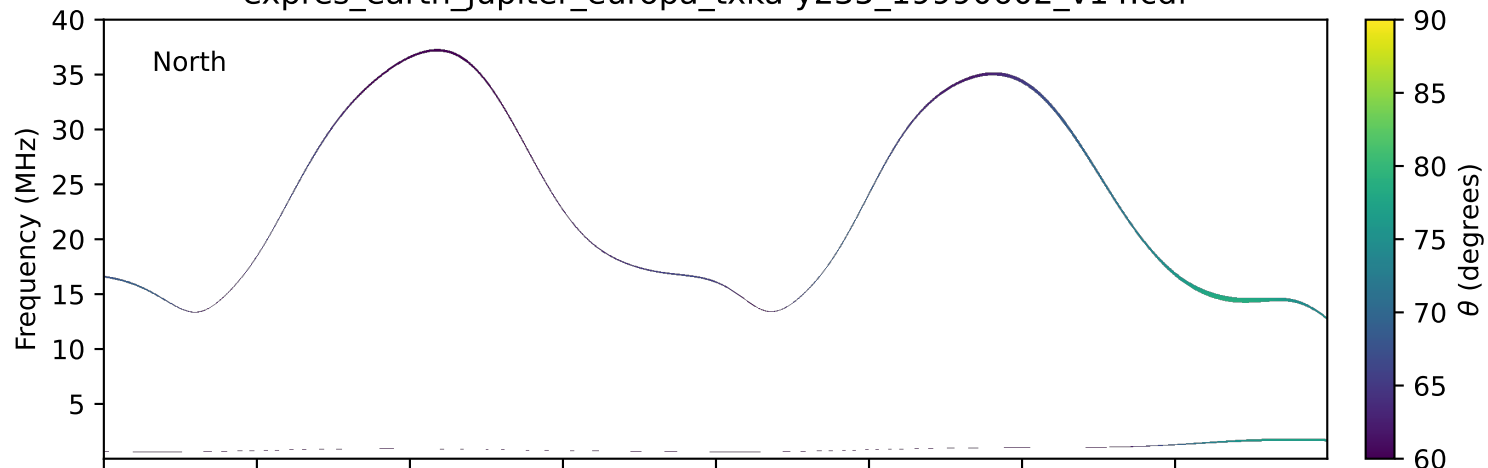
expres_earth_jupiter_europa_txka-y235_19990602_v14.cdf
