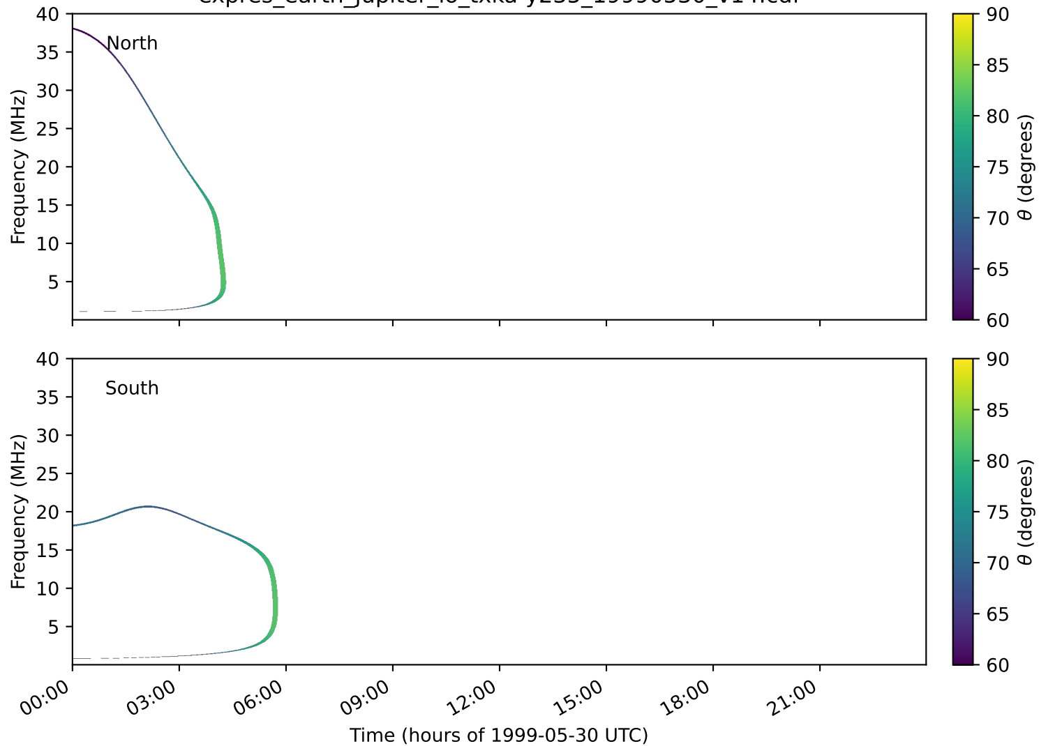
expres_earth_jupiter_io_txka-y235_19990530_v14.cdf
