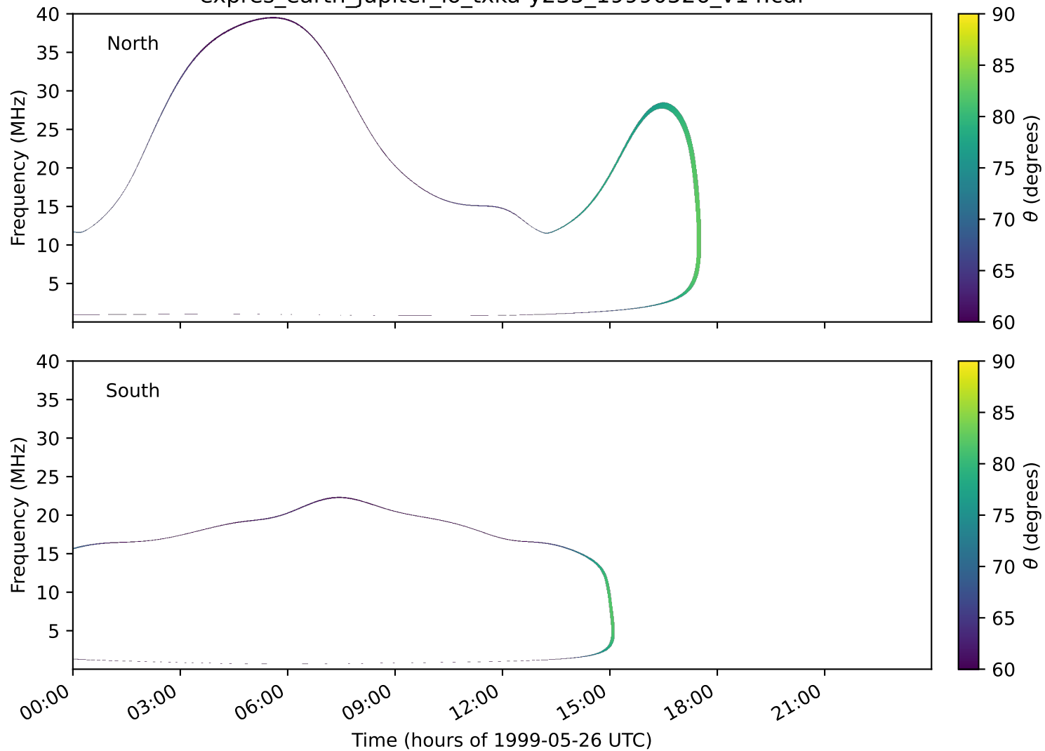
expres_earth_jupiter_io_txka-y235_19990526_v14.cdf
