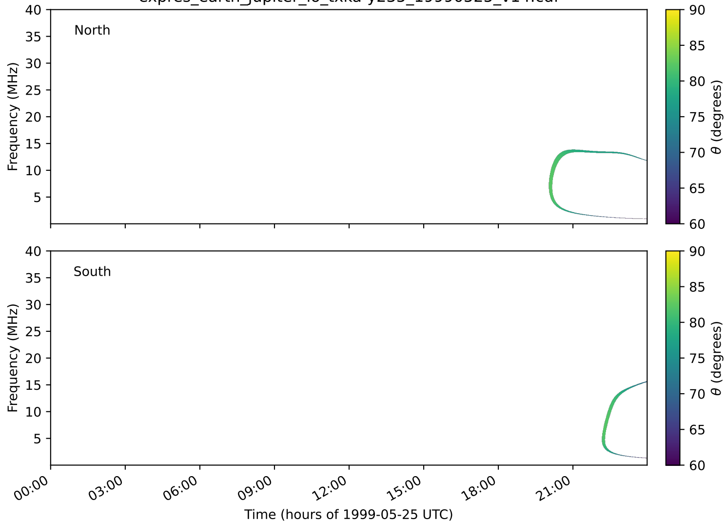
expres_earth_jupiter_io_txka-y235_19990525_v14.cdf
