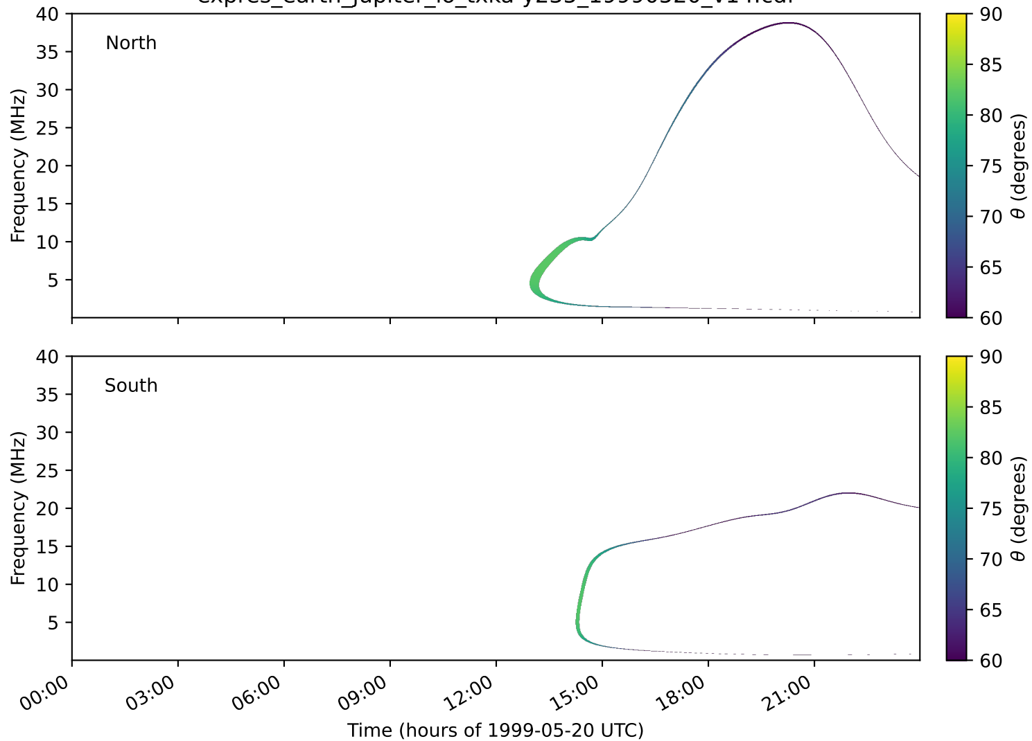
expres_earth_jupiter_io_txka-y235_19990520_v14.cdf
