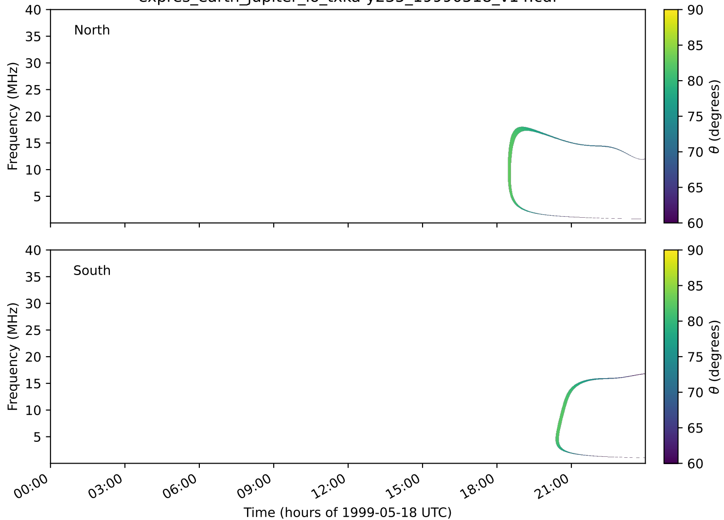
expres_earth_jupiter_io_txka-y235_19990518_v14.cdf
