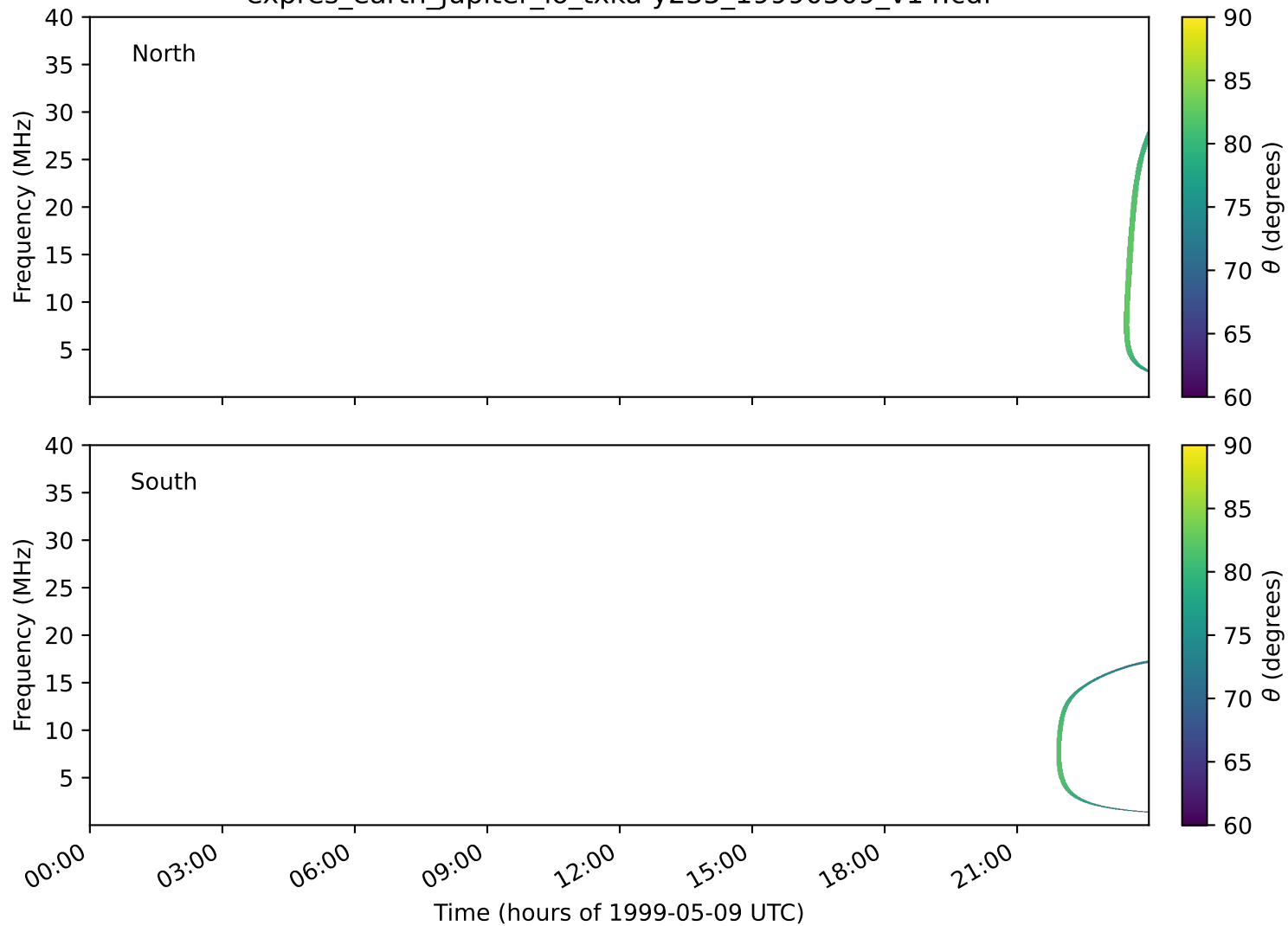
expres_earth_jupiter_io_txka-y235_19990509_v14.cdf
