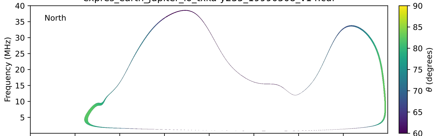
expres_earth_jupiter_io_txka-y235_19990508_v14.cdf
