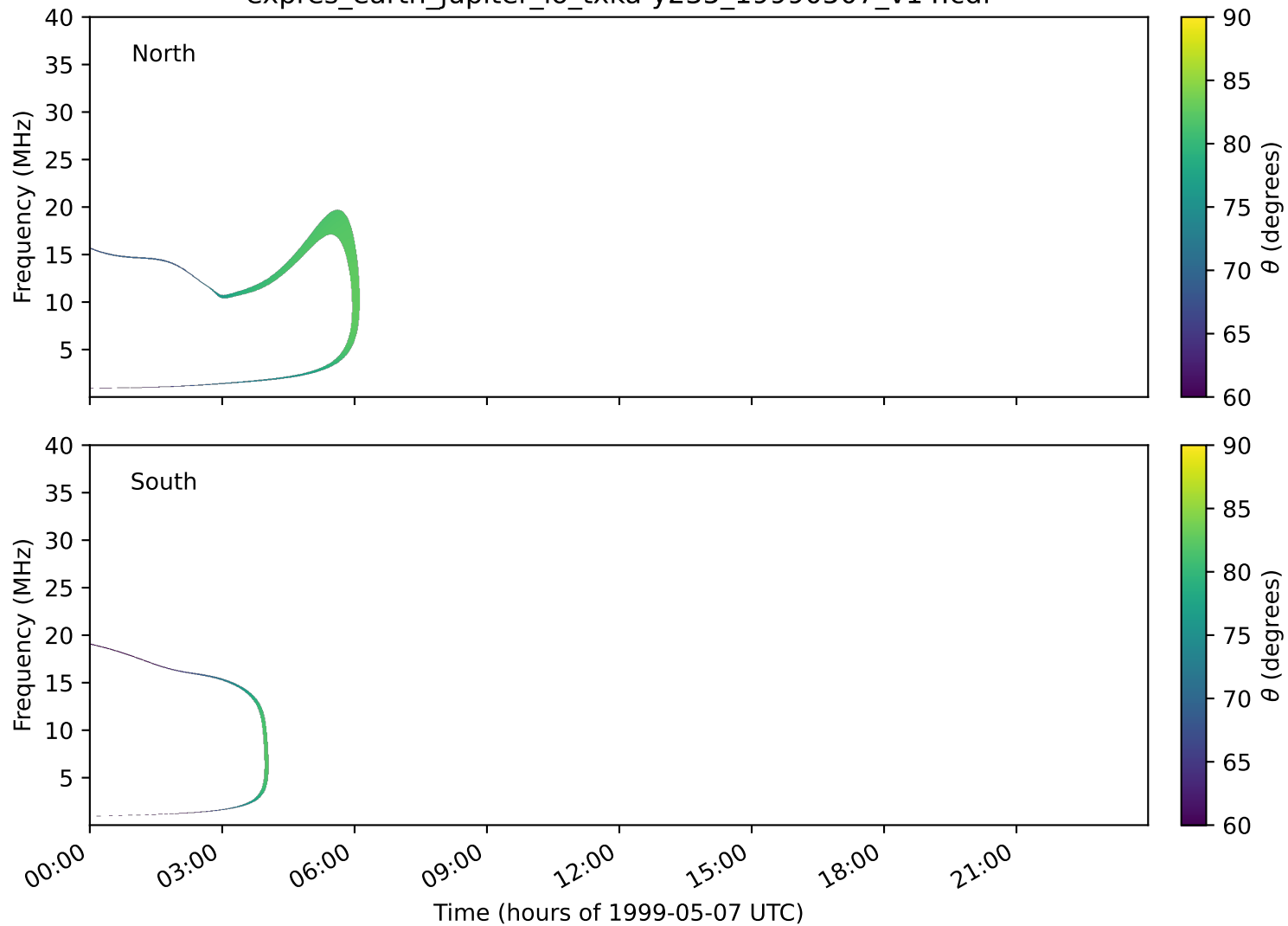
expres_earth_jupiter_io_txka-y235_19990507_v14.cdf
