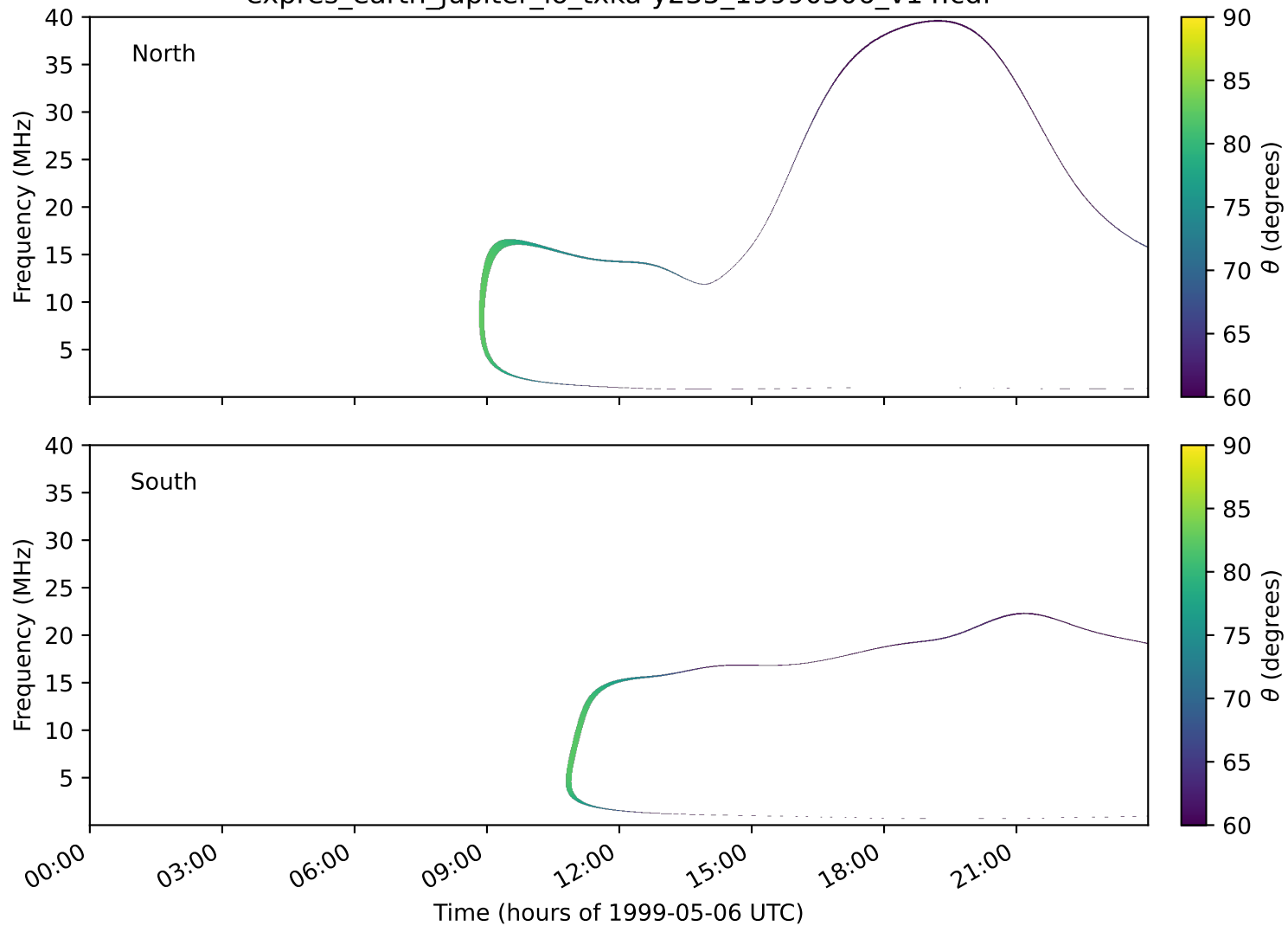
expres_earth_jupiter_io_txka-y235_19990506_v14.cdf
