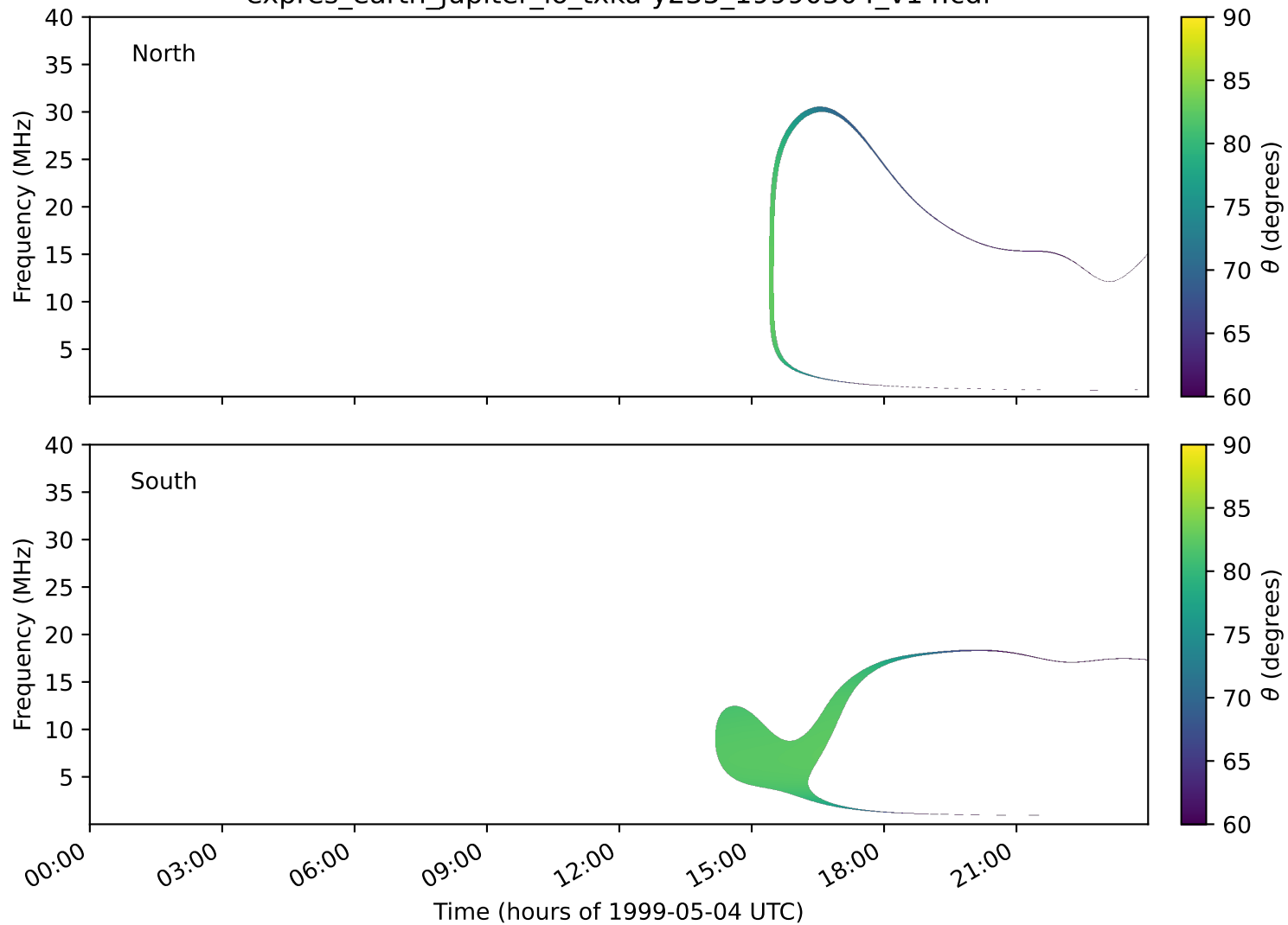
expres_earth_jupiter_io_txka-y235_19990504_v14.cdf
