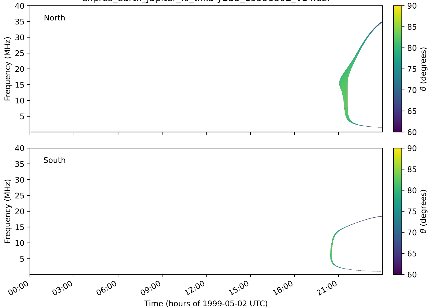
expres_earth_jupiter_io_txka-y235_19990502_v14.cdf
