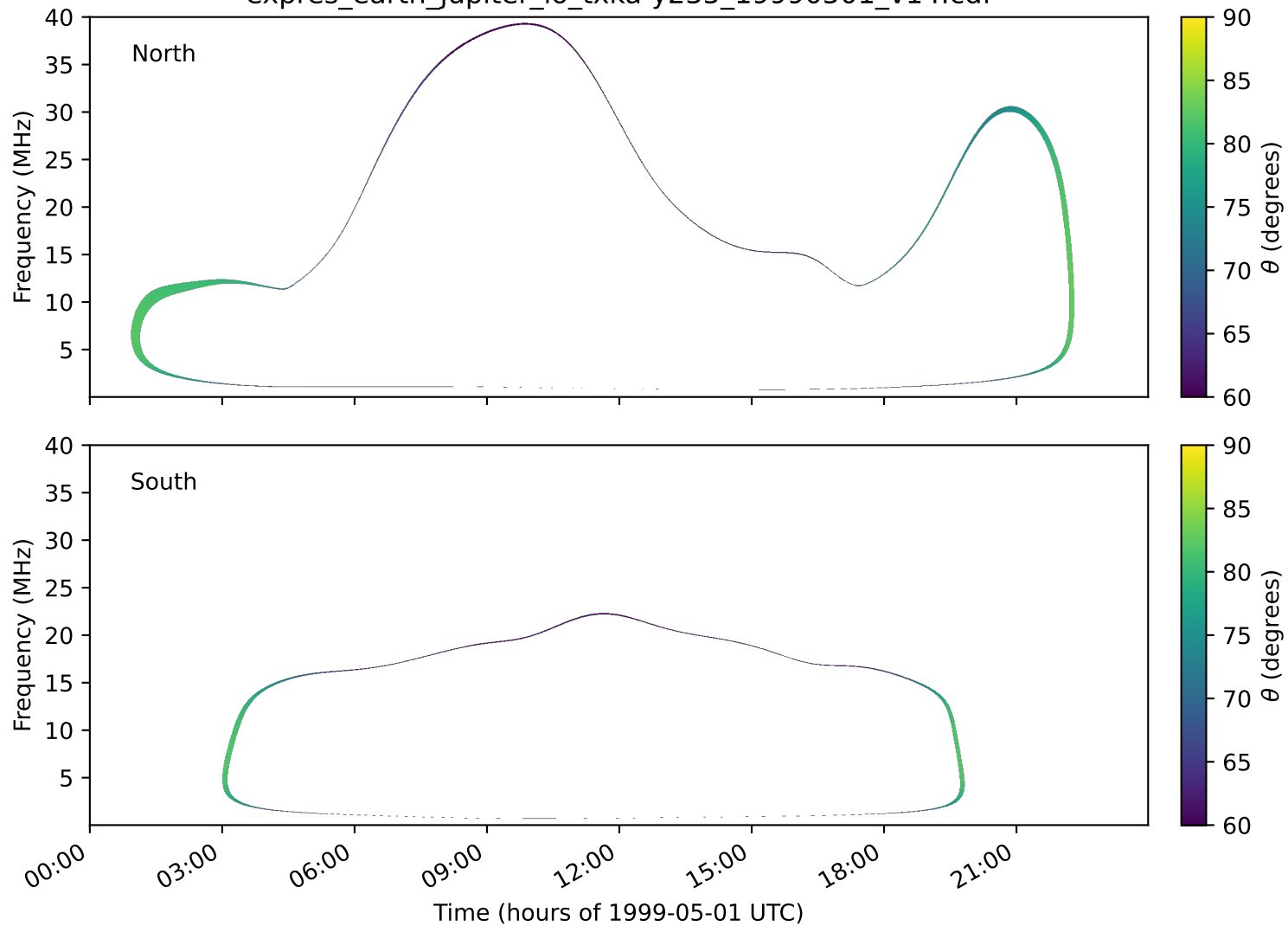
expres_earth_jupiter_io_txka-y235_19990501_v14.cdf
