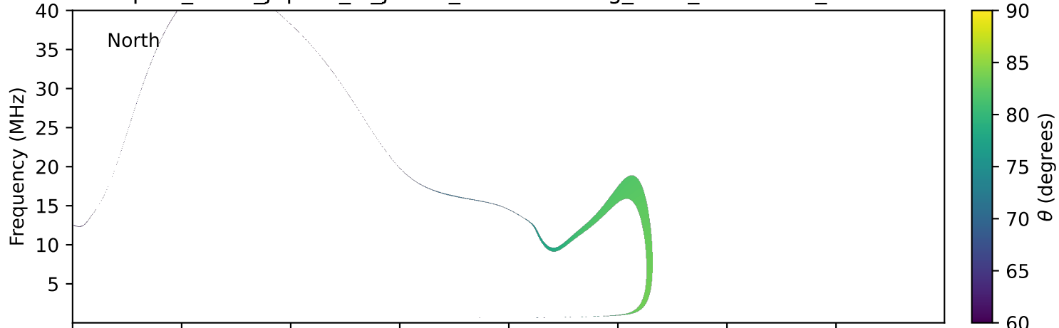
expres_earth_jupiter_io_jrm09_lossc-wid1deg_3kev_19990519_v11.cdf
