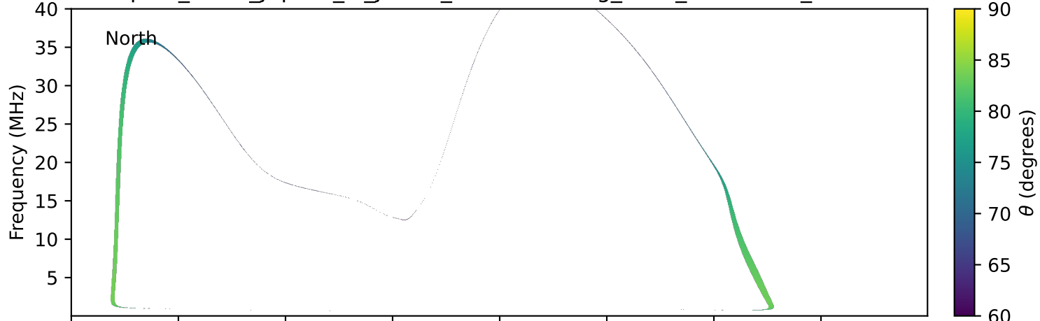
expres_earth_jupiter_io_jrm09_lossc-wid1deg_3kev_19990517_v11.cdf
