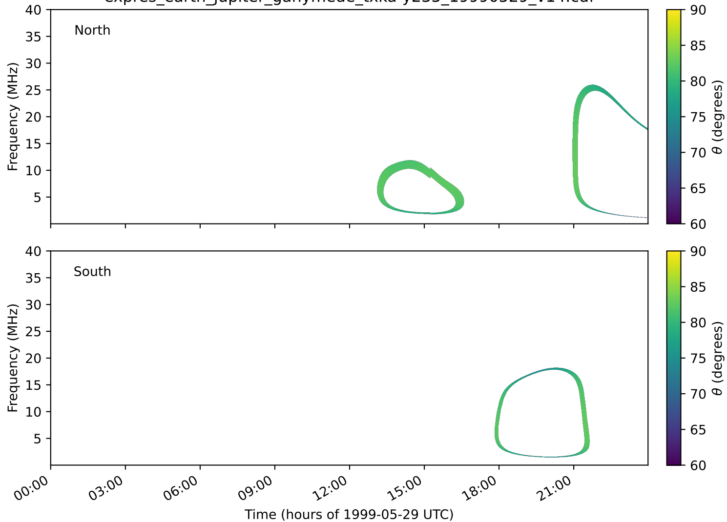
expres_earth_jupiter_ganymede_txka-y235_19990529_v14.cdf
