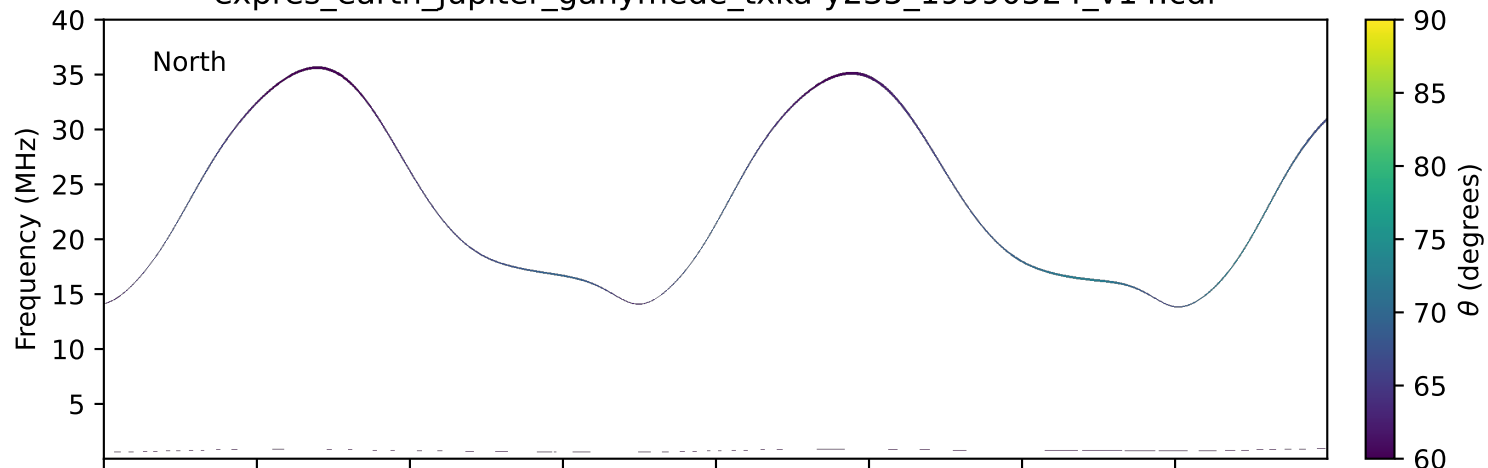
expres_earth_jupiter_ganymede_txka-y235_19990524_v14.cdf
