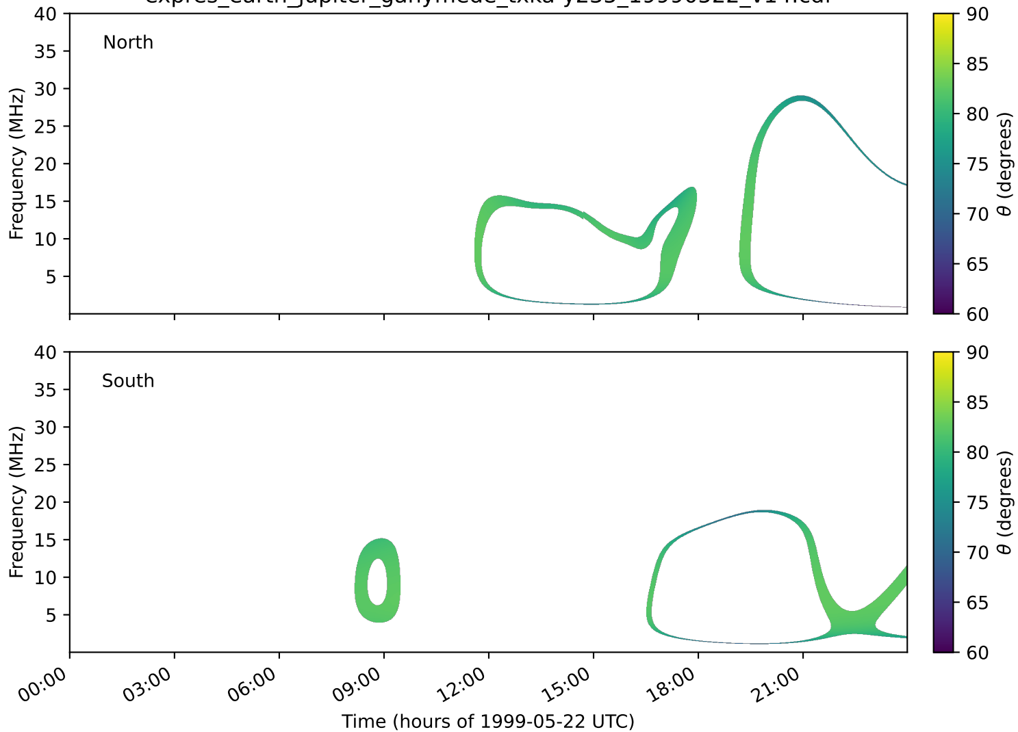
expres_earth_jupiter_ganymede_txka-y235_19990522_v14.cdf
