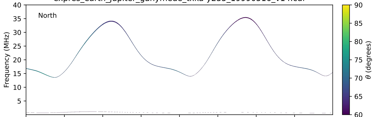
expres_earth_jupiter_ganymede_txka-y235_19990516_v14.cdf
