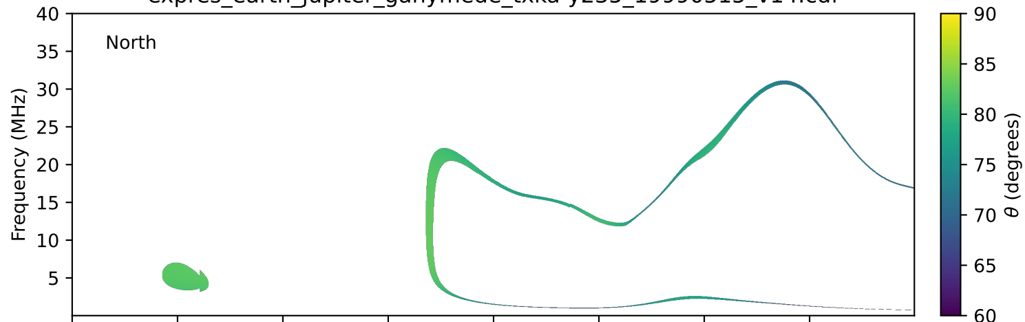
expres_earth_jupiter_ganymede_txka-y235_19990515_v14.cdf
