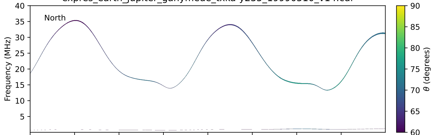
expres_earth_jupiter_ganymede_txka-y235_19990510_v14.cdf
