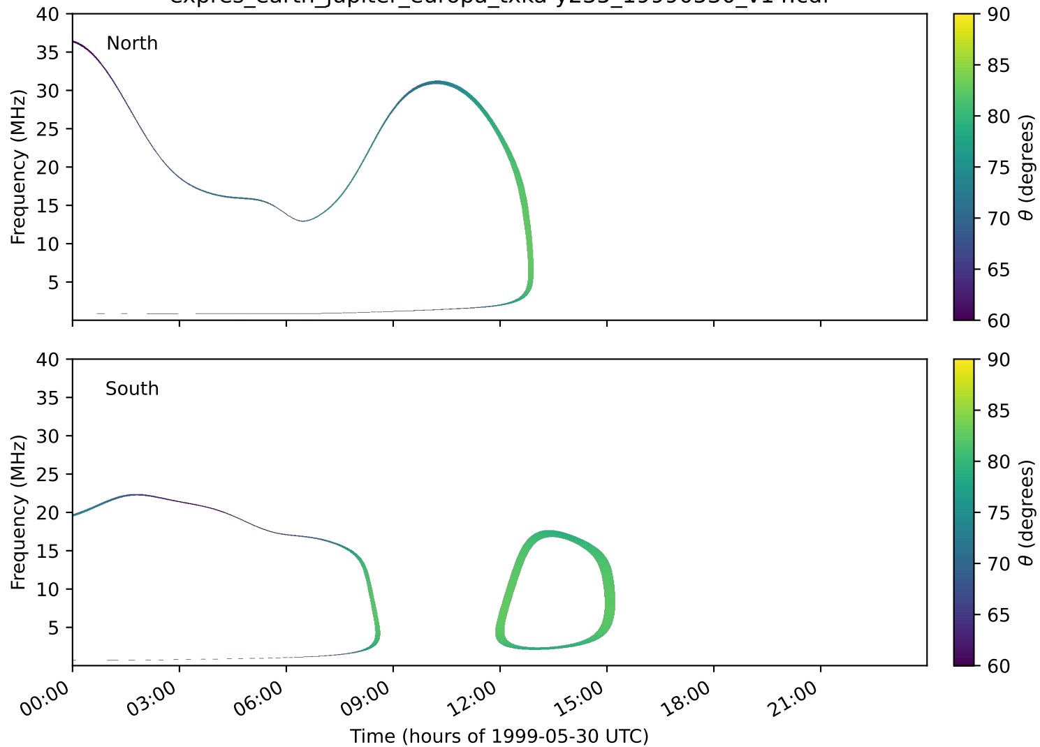
expres_earth_jupiter_europa_txka-y235_19990530_v14.cdf
