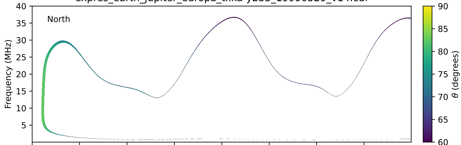
expres_earth_jupiter_europa_txka-y235_19990529_v14.cdf
