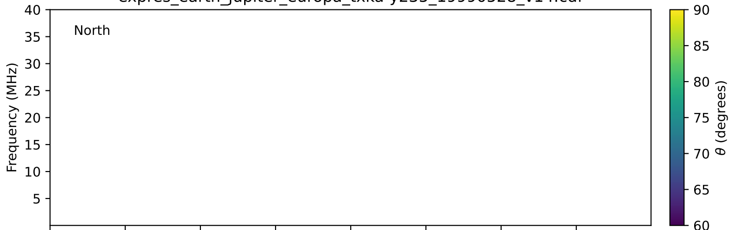
expres_earth_jupiter_europa_txka-y235_19990528_v14.cdf
