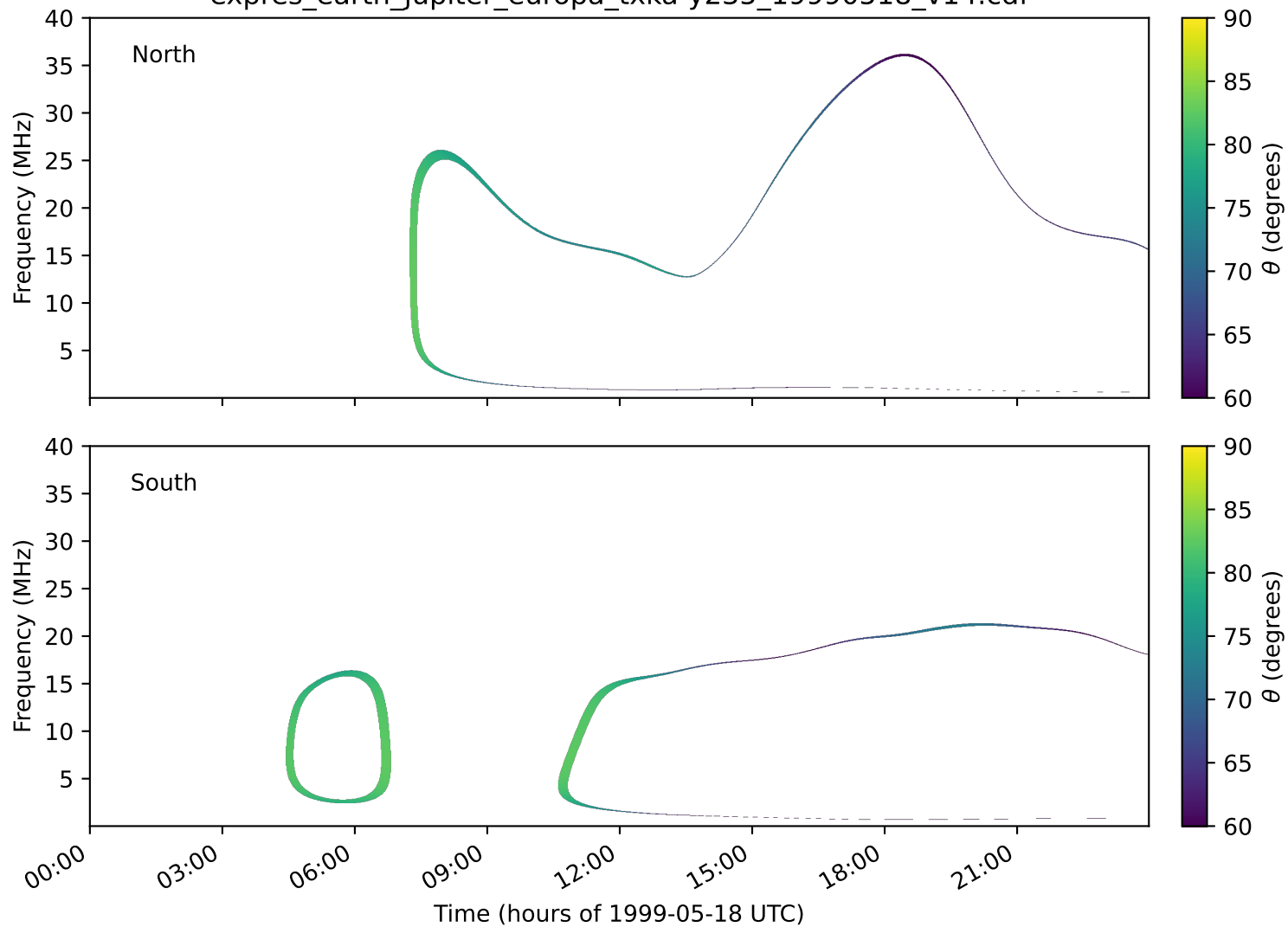
expres_earth_jupiter_europa_txka-y235_19990518_v14.cdf
