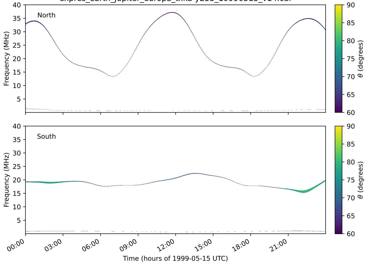
expres_earth_jupiter_europa_txka-y235_19990515_v14.cdf
