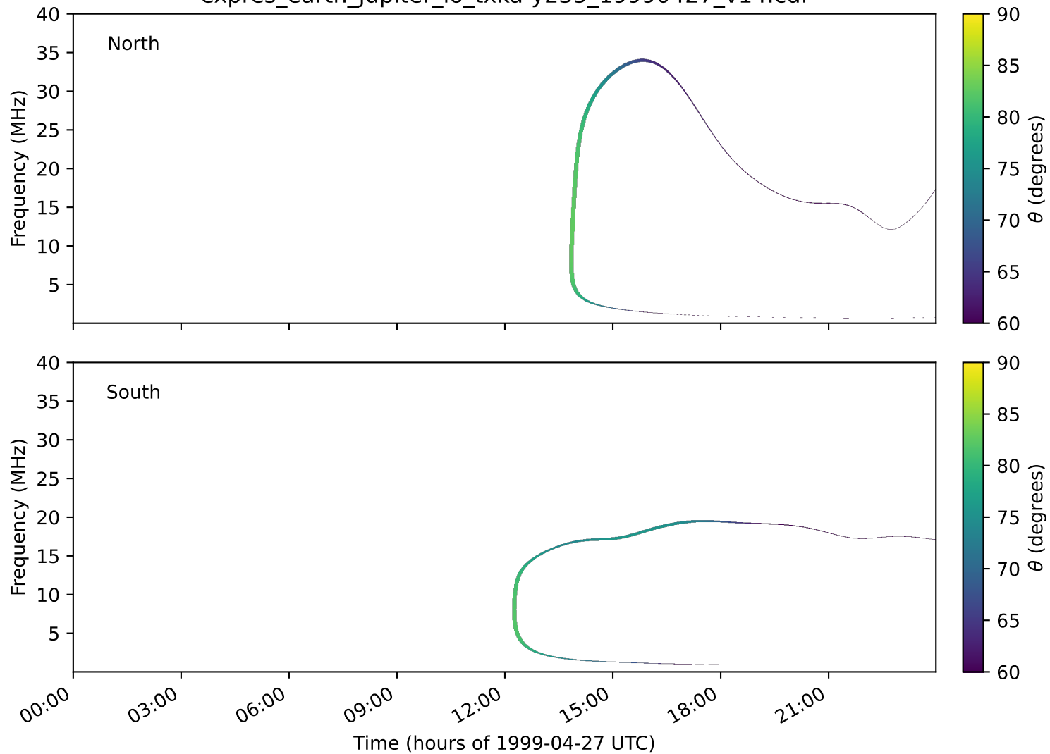
expres_earth_jupiter_io_txka-y235_19990427_v14.cdf
