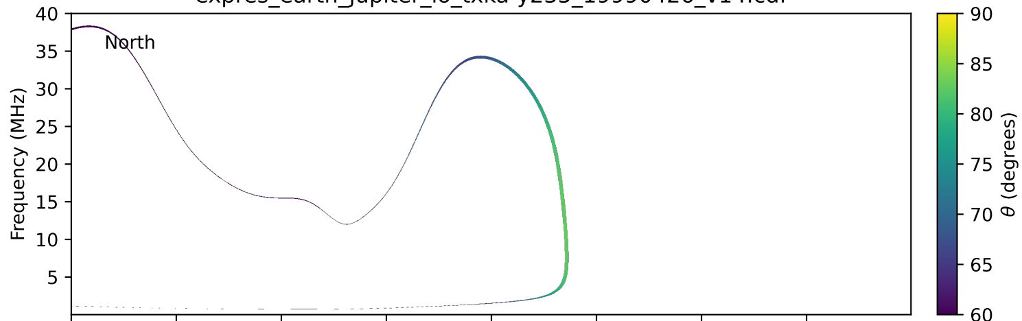
expres_earth_jupiter_io_txka-y235_19990426_v14.cdf
