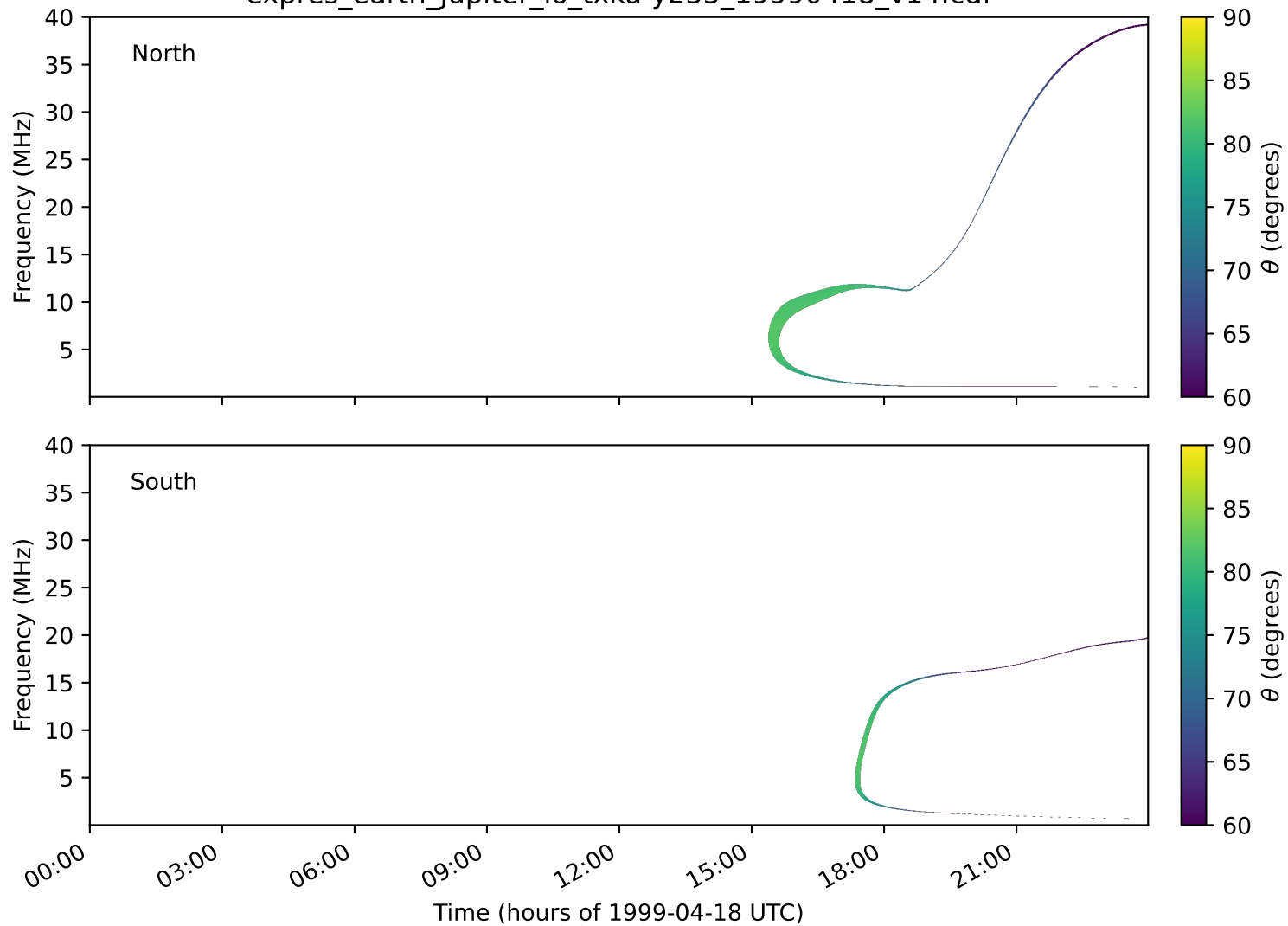
expres_earth_jupiter_io_txka-y235_19990418_v14.cdf
