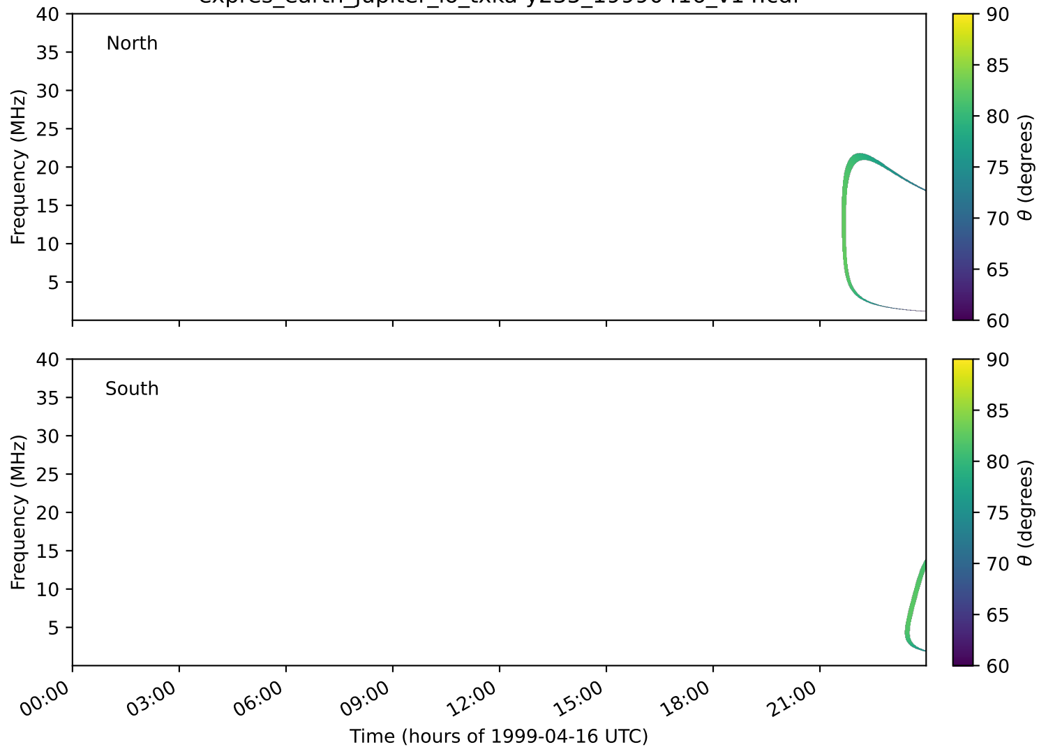
expres_earth_jupiter_io_txka-y235_19990416_v14.cdf
