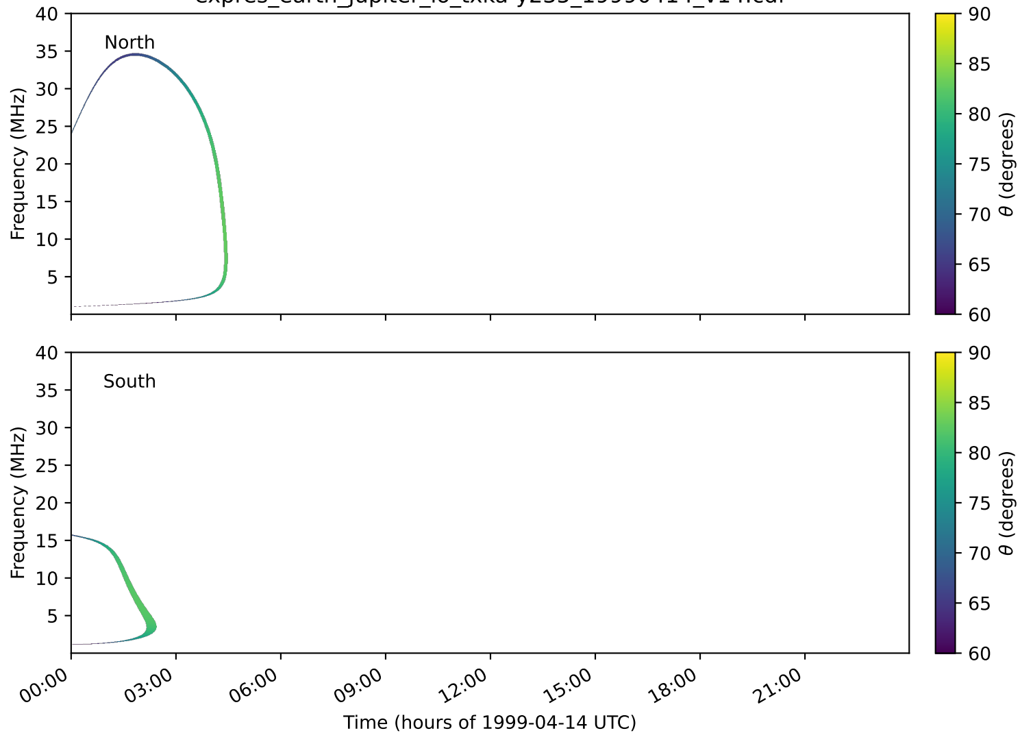
expres_earth_jupiter_io_txka-y235_19990414_v14.cdf
