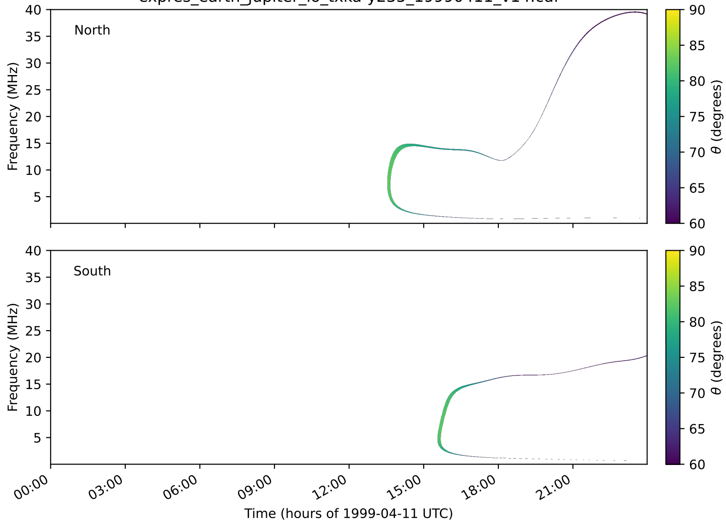
expres_earth_jupiter_io_txka-y235_19990411_v14.cdf
