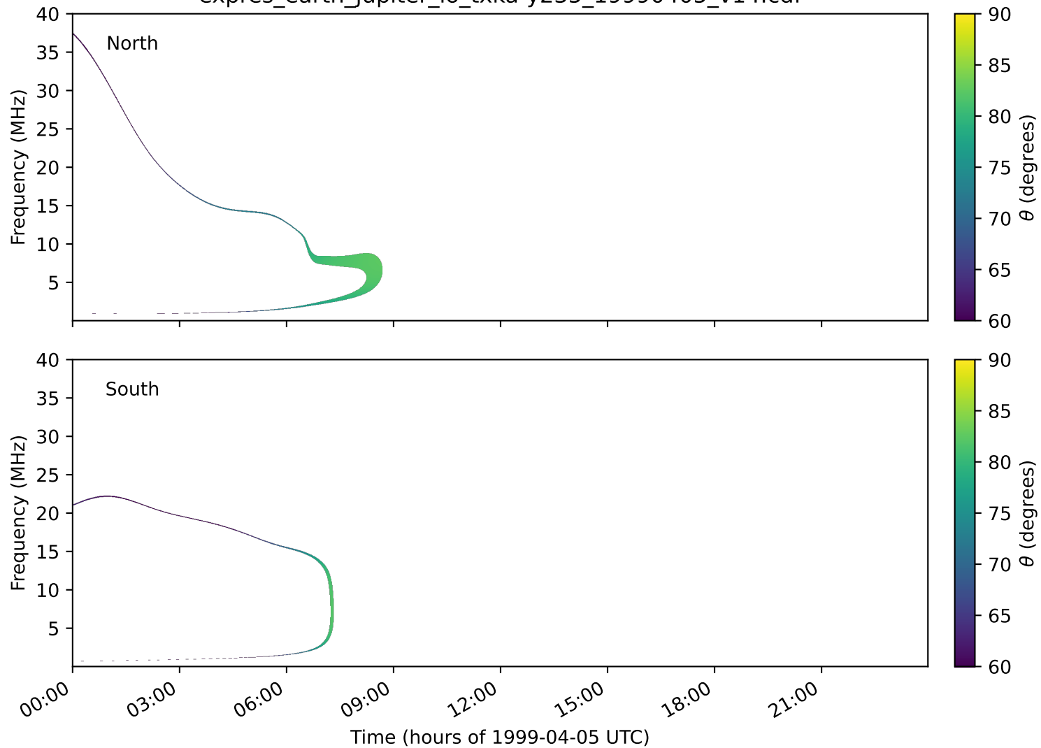
expres_earth_jupiter_io_txka-y235_19990405_v14.cdf
