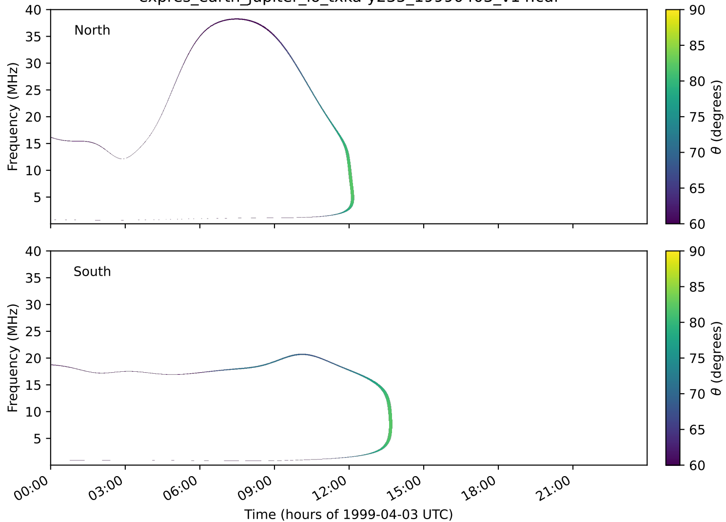
expres_earth_jupiter_io_txka-y235_19990403_v14.cdf
