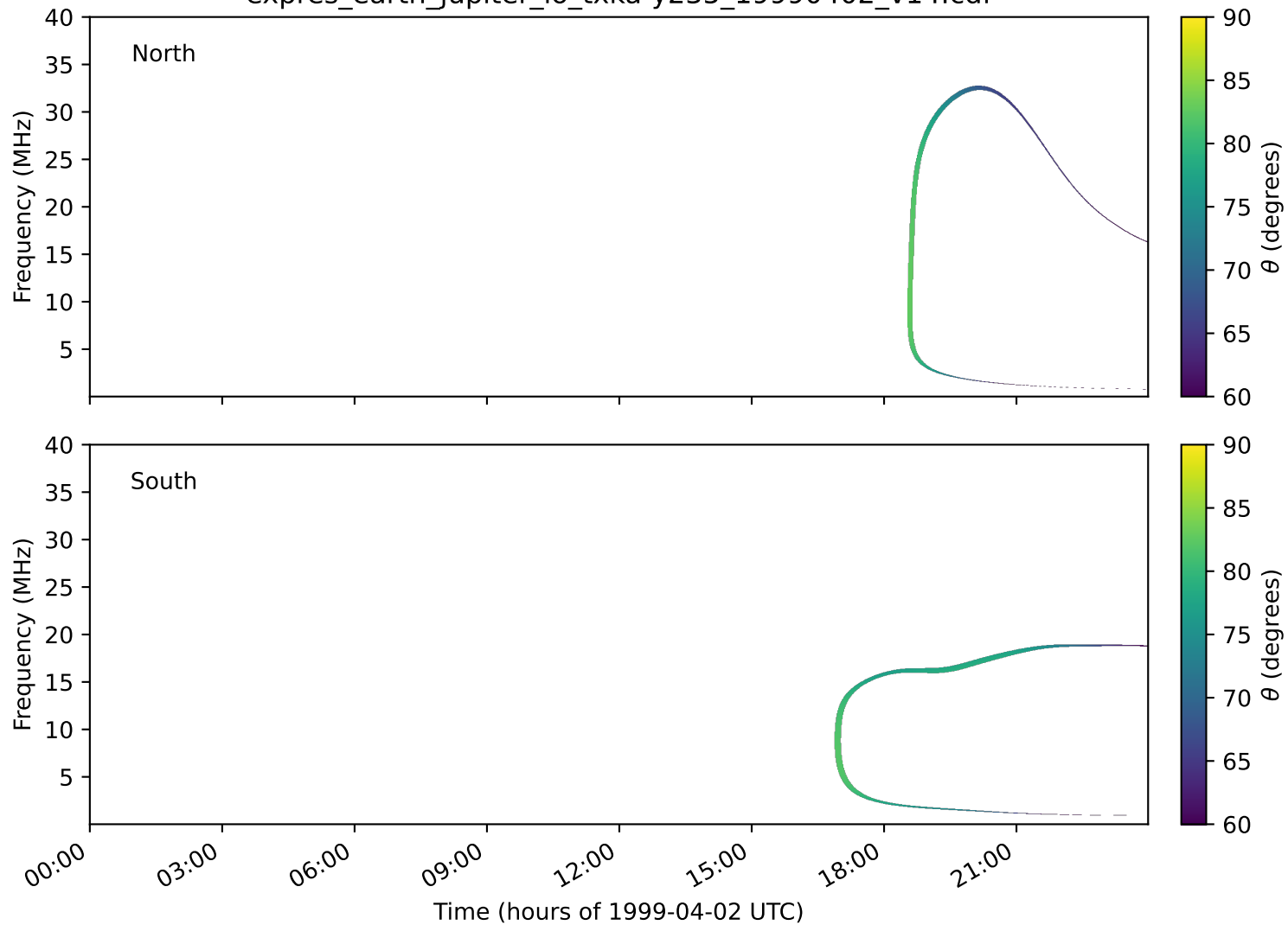
expres_earth_jupiter_io_txka-y235_19990402_v14.cdf
