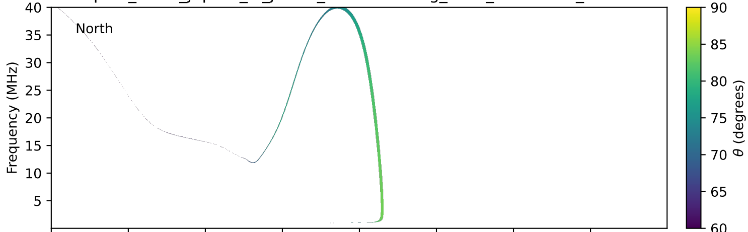
expres_earth_jupiter_io_jrm09_lossc-wid1deg_3kev_19990419_v11.cdf
