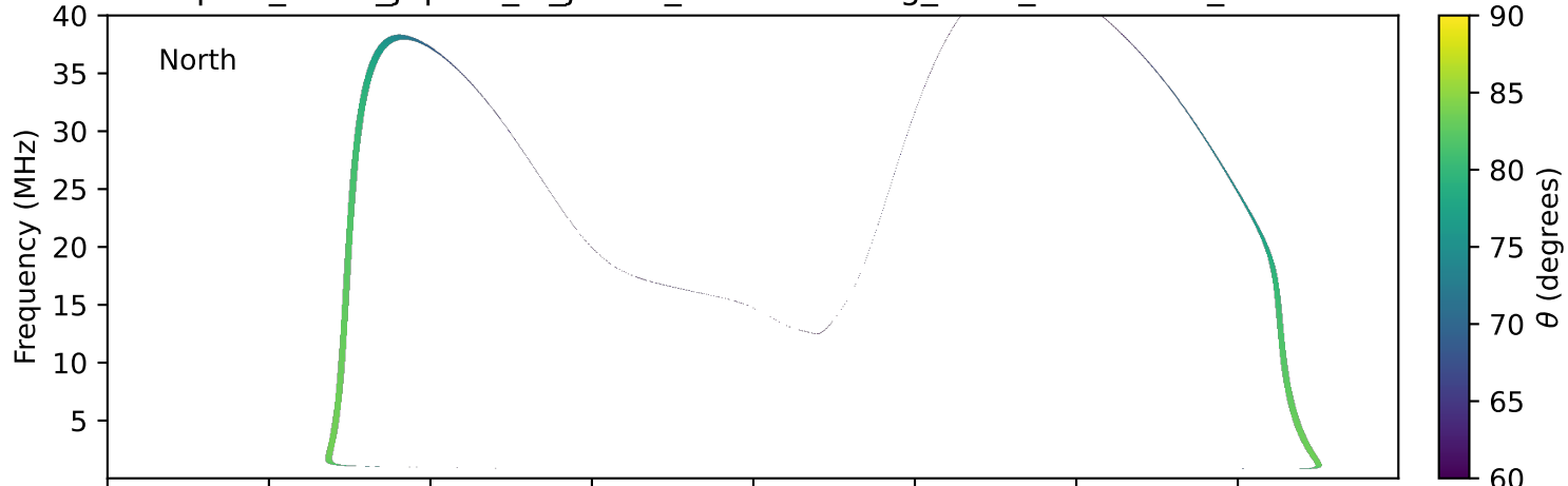
expres_earth_jupiter_io_jrm09_lossc-wid1deg_3kev_19990415_v11.cdf
